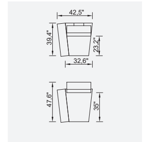
Angled Module (Left)
